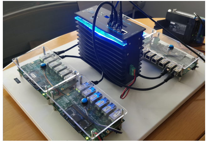
Fig. 2. The hardware demo setup
