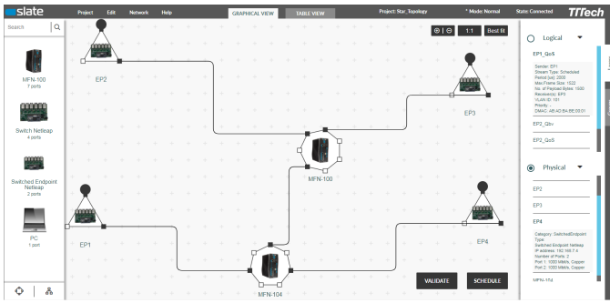
Fig. 1. Slate XNS - A Browser-based TSN Scheduling Tool
